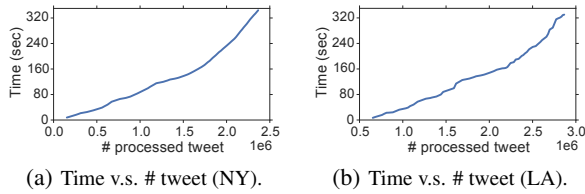
Figure 10: Throughput of activity timeline construction.
